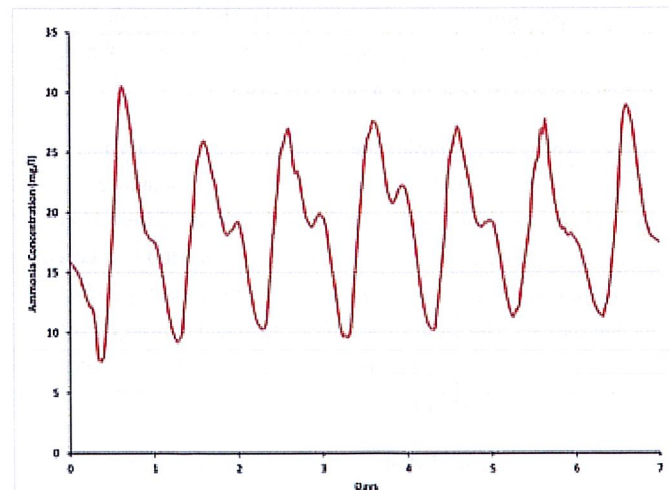
Figure 1: Seven days of influent ammonium readings.
