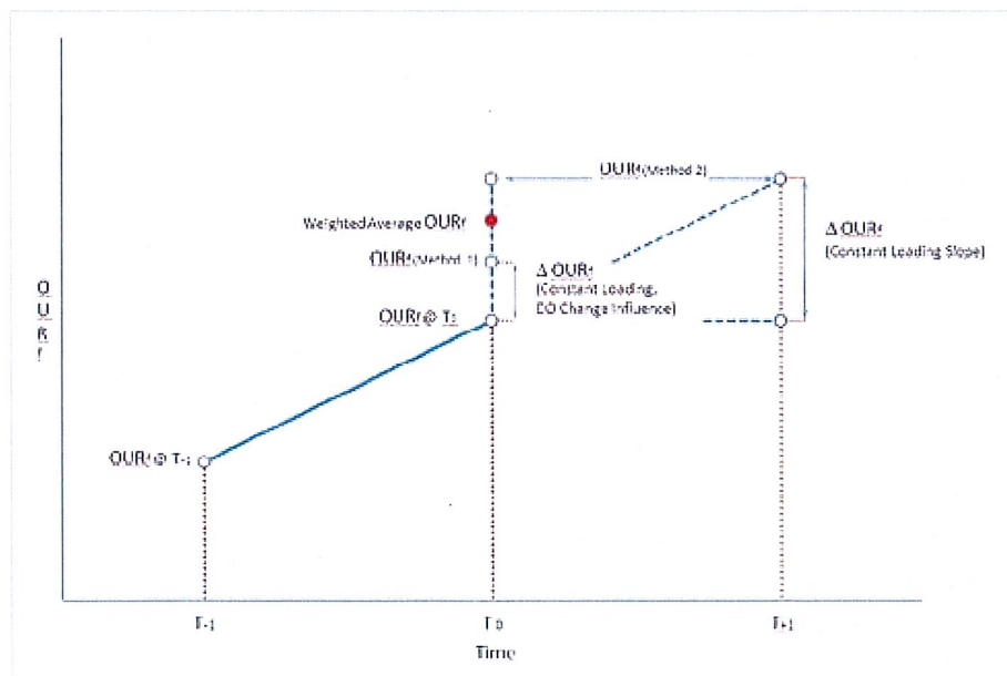
Figure 4: Graphical depiction of OURf airflow calculation methods.
