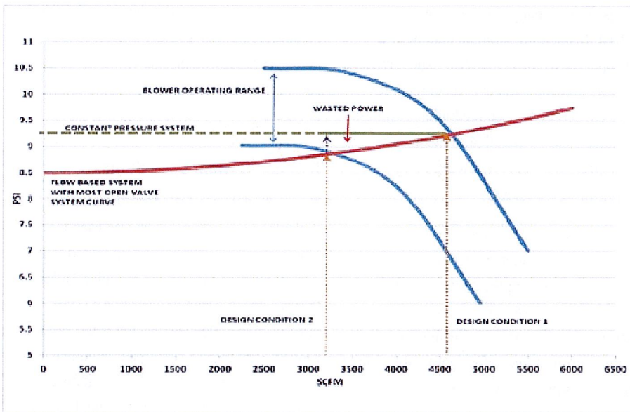
Figure 3: Pressure versus flow-based blower control.
