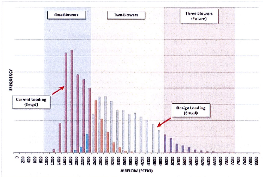
Figure 2: Airflow histogram with blower range.
